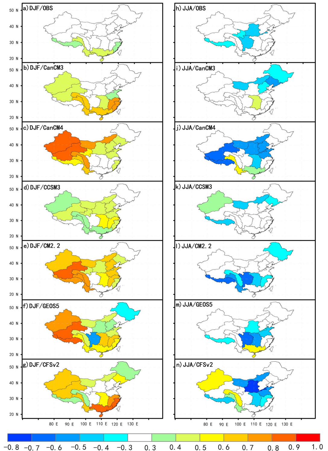
Figure 4. (a–n) The spatial distributions of correlations between regional mean SPI3 and Niño 3.4 SST anomaly from observations and NMME seasonal climate forecasts at lead-1 seasons during DJF and JJA. Values between -0.3 and 0.3 are insignificant and masked out.
