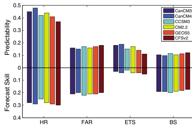
Figure 7. Hit rate (HR), false alarm rate (FAR), Equitable Threat Score (ETS), Brier Score (BS) for predictability and forecast skill for drought events ( SPI3 < -0.8 ) at lead-0 seasons.
