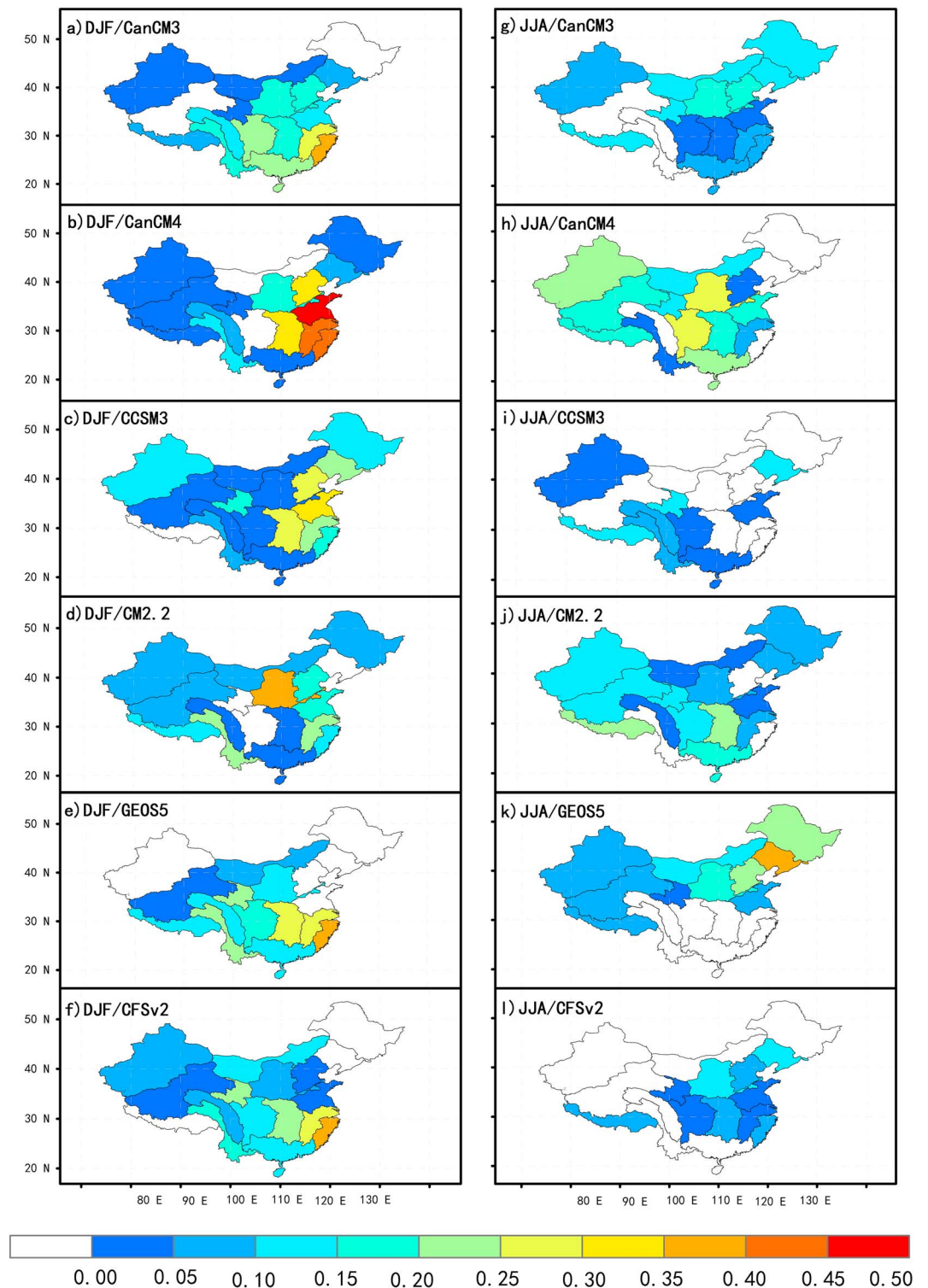
Figure 3. SPI3 forecast skill in terms of anomaly correlation (AC) at lead-1 seasons for 17 hydroclimate regions in China during DJF and JJA.
