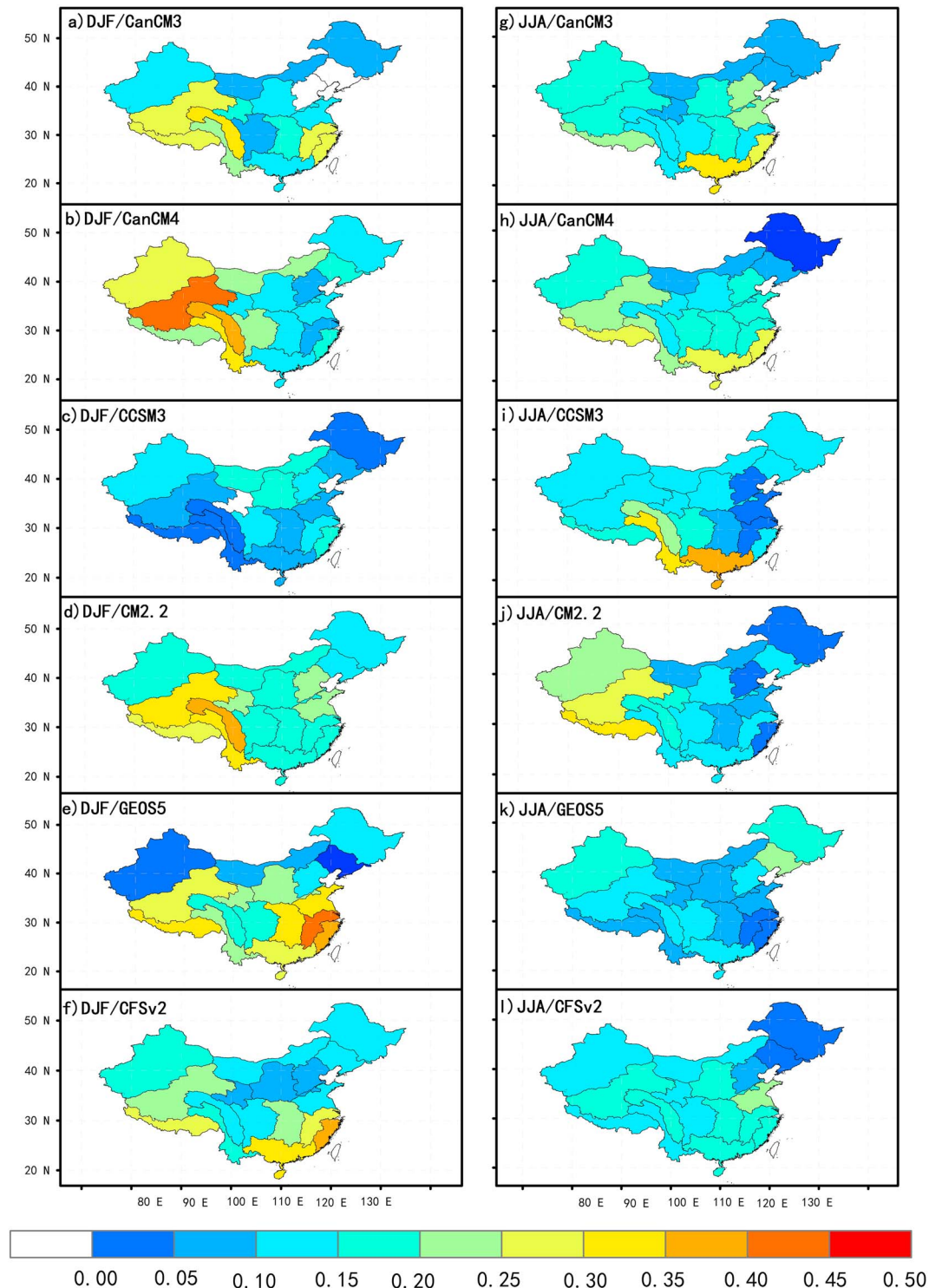
Figure 2. SPI3 predictability in terms of anomaly correlation (AC) at lead-1 seasons for 17 hydroclimate regions in China during DJF and JJA.
