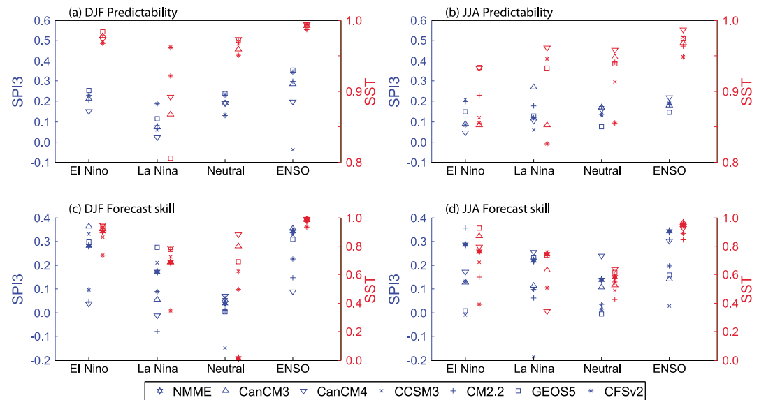
Figure 5. The (a and b) predictability and (c and d) forecast skill in terms of anomaly correlation (AC) for the SPI3 and SST in different ENSO phases over ENSO-affected river basins during DJF (Figures 5a and 5c) and JJA (Figures 5b and 5d). The blue color refers to SPI3, and the red color refers to SST.
