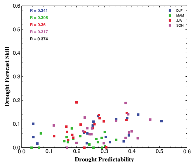
Figure 6. The same as Figure 1 but for drought (SPI3 < −0.8) predictability (x axis) versus forecast skill (y axis) at lead-0 seasons.
