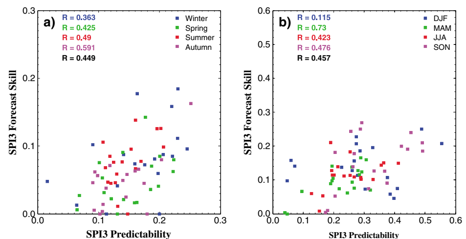
Figure 1. SPI3 predictability (x axis) versus forecast skill (y axis) in terms of Anomaly Correlation (AC) at (a) lead-1 seasons and (b) lead-0 seasons. Colors represent seasons: blue for boreal winter seasons (November–January, December–February, and January–March), green for spring seasons (February–April, March–May, and April–June), red for summer seasons (May–July, June–August, and July–September), and orange for autumn seasons (August–October, September–November, and October–December).
